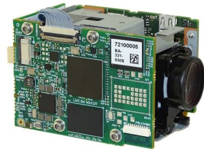
Figure 1. Harrier 10x AF-Zoom IP Camera (Tamron MP3010M-EV)
