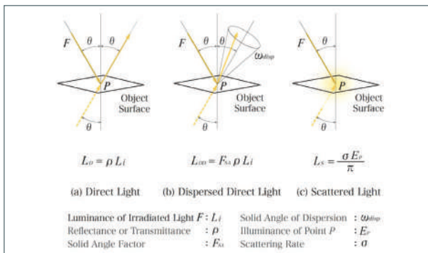
The classification of object light and its luminance
